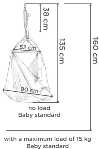
Figure 3 : DIMENSIONS OF THE CRADLE WITH SPRING UNDER DIFFERENT LOADS
